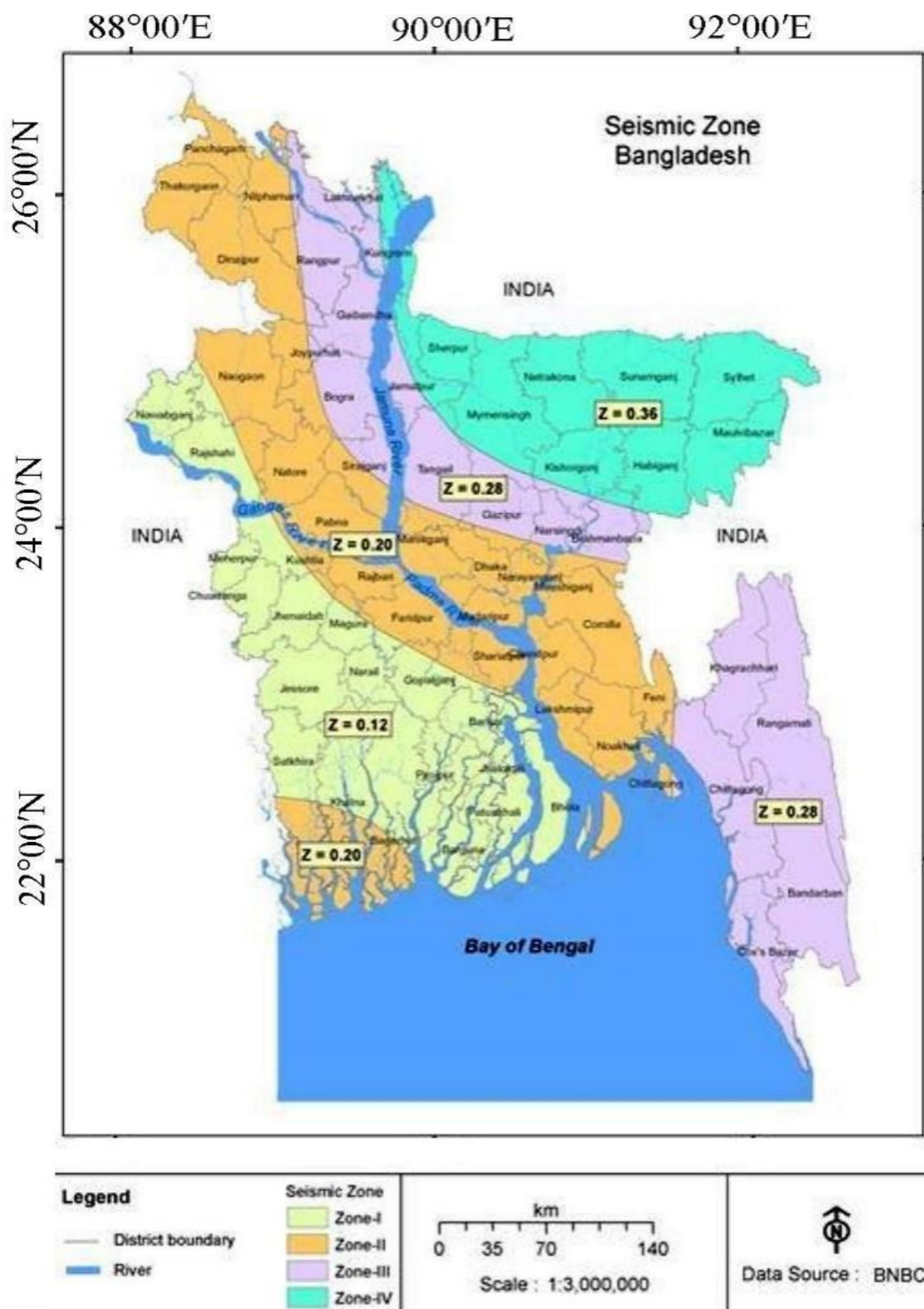
Figure 3: Seismic zone in Bangladesh Map BNBC-2020
